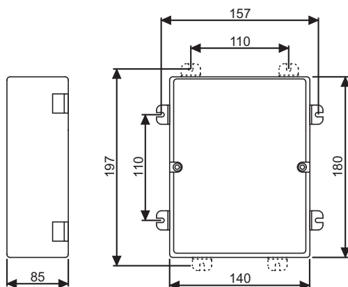
Fig.1 - ENCOMBREMENT (mm):
