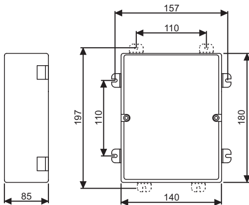
Fig.1 - DIMENSIONS (mm):
